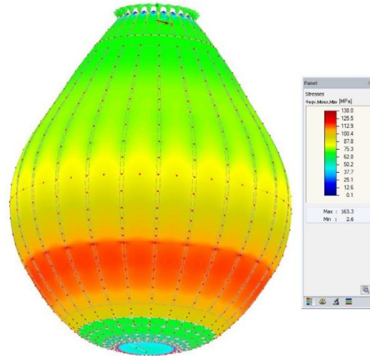
Figure 12 - 35 Tonne Equivalent von-Mises Stress
