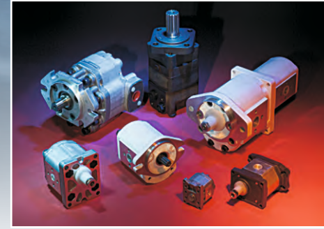
Gear Pumps/Gear Motors
